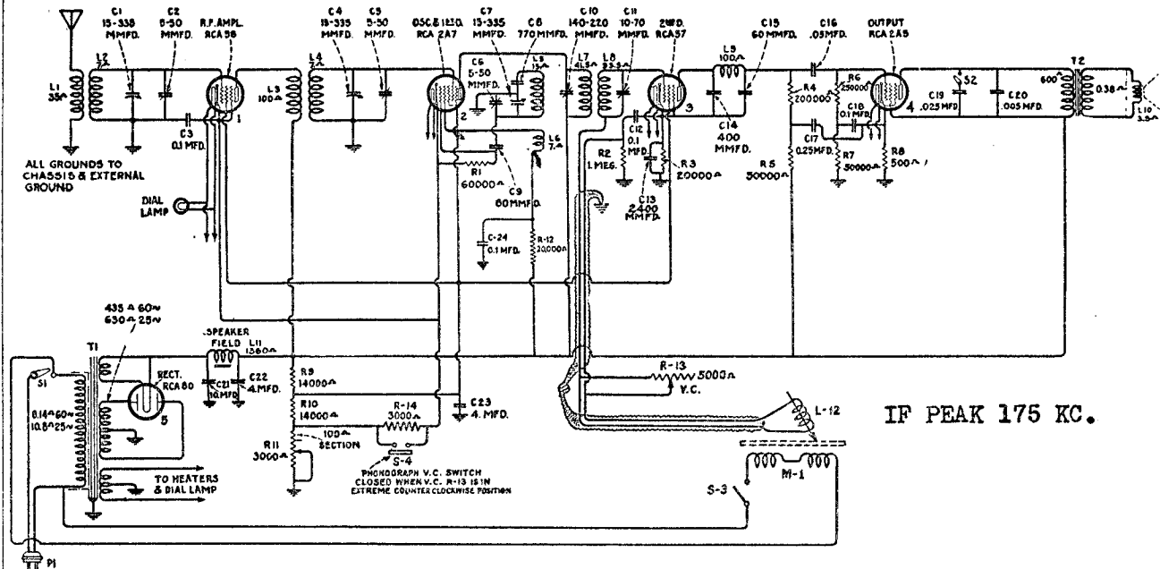
Figure C—Schematic Circuit
